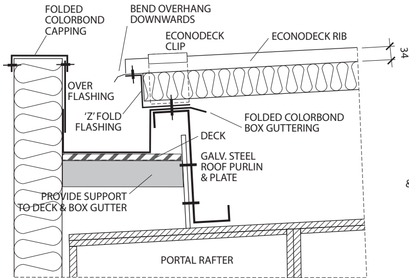
BOX GUTTER DETAIL
