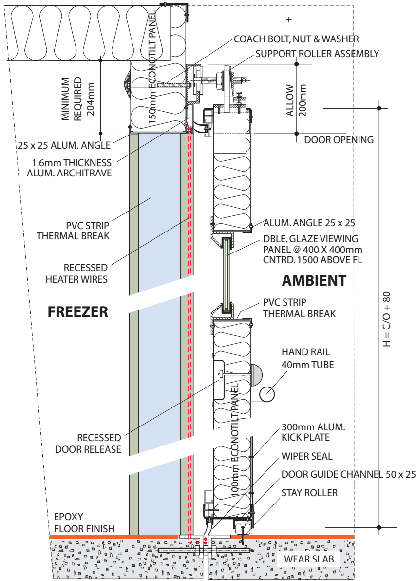
CROSS SECTION SCALE 1:10
